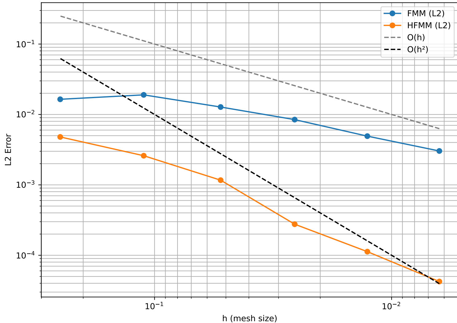
FMM Convergence - Square with Hole
